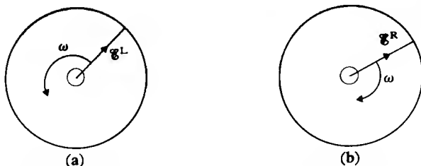
4.2 In circularly polarised radiation the electric field vectors \mathfrak{E}^L , and \mathfrak{E}^R rotate in anticlockwise and clockwise directions when facing into the oncoming wave.
